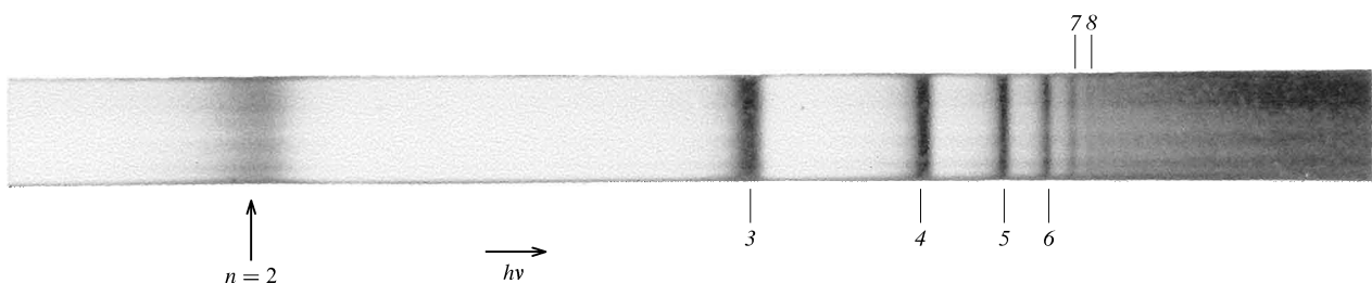
Figure 1. Optical spectrum of an exciton in cuprous oxide, showing the yellow–orange part of the visible spectrum.
