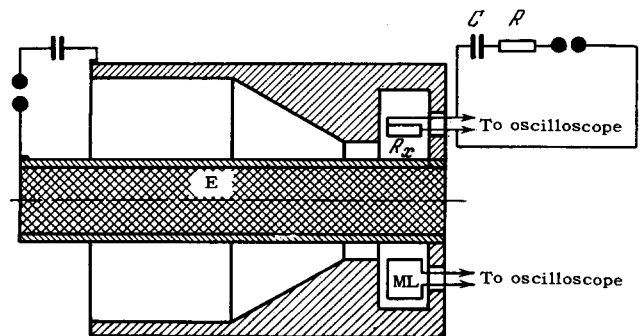
FIG. 9. Diagram of experiment on the measurement of the resistance of graphite. R_x —sample, ML—loop for measuring H; RC \gg rise time of H.
