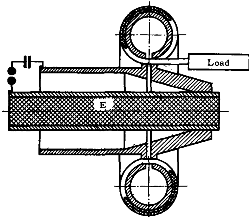
FIG. 5. MC transformer system.
