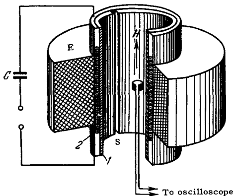
FIG. 1. Diagram of MK-1 generator.
