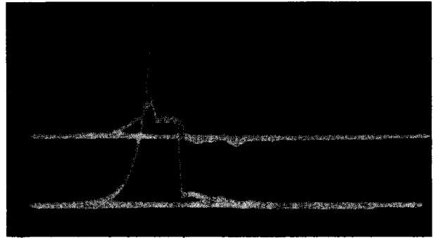
FIG. 7. Oscillogram showing the magnetic field intensity. Beam 1—background (signal from shorted wires); beam 2—signal from measuring turn (integration with RC network).
