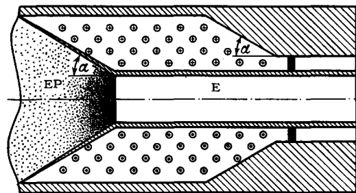
FIG. 11. Diagram of setup for launching a ring.
