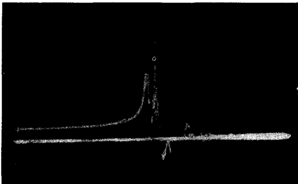
FIG. 10. Oscillogram of voltage on graphite sample.
