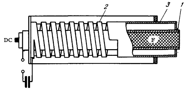
FIG. 3. Diagram of MK-2 generator.
