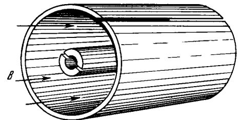
FIG. 8. Magnetic-field concentrator.
