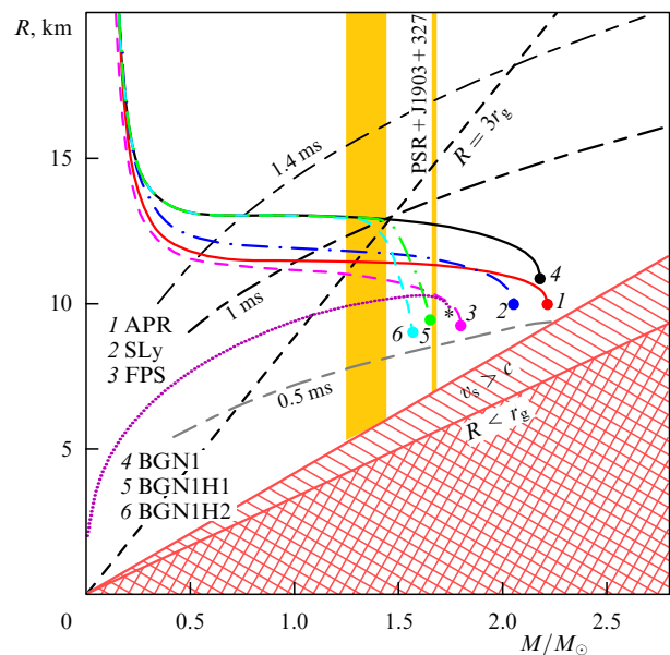
Figure 4. Mass dependence of the compact star radius. Curves 1–6 correspond to the equations of state of neutron stars shown in Figs 2 and 3. The dotted curve corresponds to one of the feasible equations of state of a quark star. The hatched triangular area is forbidden by the causality principle. The crosshatched triangular area lies below the event horizon. Three short- and long-dashed curves show additional constraints for rotating neutron stars: the area under the corresponding curve is permitted at the rotation periods indicated (1.4, 1, and 0.5 ms). The straight line R = 3r_g corresponds to the minimal stability radius of the circular orbit of a test particle around the neutron star of a given mass. The wide vertical strip encompasses the masses of binary neutron stars measured with an error less than 0.1M_\odot at the 2\sigma level [25]; the narrow vertical strip corresponds to the mass of the PSR J1903 + 0327 millisecond pulsar [42] (see the Note added in proof).
