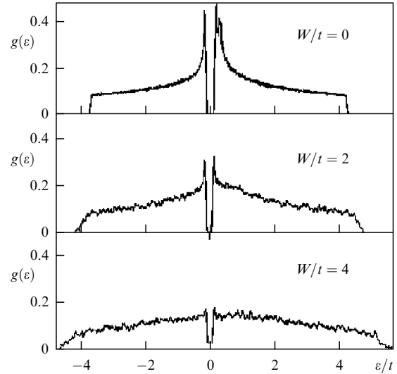
Figure 12. Density g(\epsilon) of single-particle states on a 24 \times 24 lattice at three levels of disorder W/t and an average electron density \langle n \rangle = 0.875 [63].
