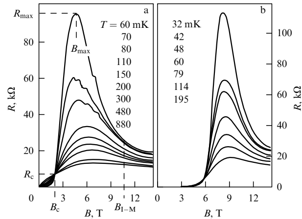
Figure 26. Families of R(B) isotherms for two close states of an amorphous In–O film 200 Å thick in fields (a) perpendicular and (b) parallel to the film [108]. The position of the point of intersection of the isotherms in figure (a) determines the critical values of R_c and B_c ; the meaning of the field B_{I-M} is explained in Fig. 27 and in the main text.
