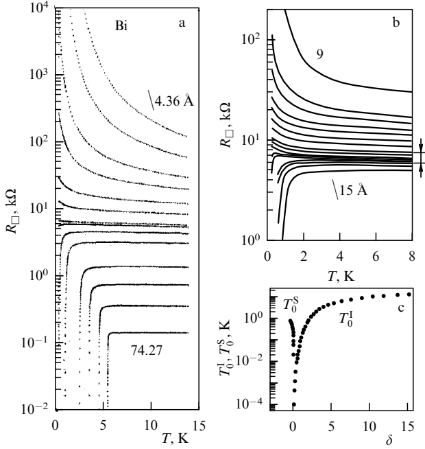
Figure 18. (a) Evolution of the temperature dependences of the resistance of amorphous Bi films deposited on a Ge underlayer of thickness b_0 = 6 \text{ \AA} with film thickness b increasing from above downward [83]. (b) Central part of an analogous series of R(T, b = \text{const}) curves on an enhanced scale and with a smaller step in b on the interval of thicknesses b from 9 to 15 \text{\AA} ; the films were deposited over a Ge underlayer 10 \text{\AA} thick onto the (100) surface of an \text{SrTiO}_3 single crystal [84]. (c) Characteristic scaling parameters T_0^I and T_0^S on each side of the quantum phase transition; the quantity \delta plotted on the abscissa represents normalized difference between the film resistance R^* and the critical value R_c^* at T^* = 14 \text{ K} : \delta = (R^* - R_c^*)/R_c^* [85].
