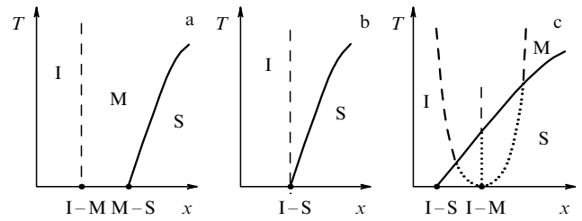
Figure 2. Variants of the phase diagram with transitions between three different states of the electron system: insulator (I), normal metal (M), and superconductor (S). The quantum transitions are shown by dots lying on the abscissa; the thermodynamic transitions, by solid curves; the cross-overs and the boundaries of the critical region, by dashed lines, and the virtual boundaries in figure (c), by dotted lines.
