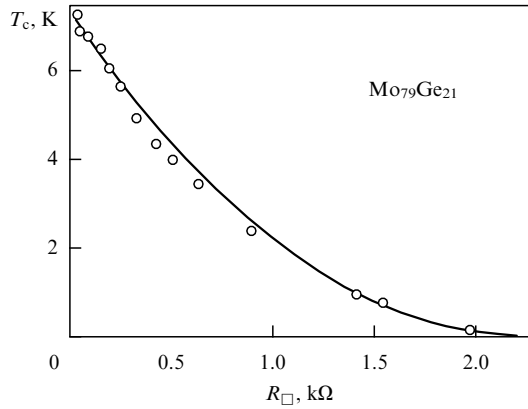
Figure 7. Suppression of superconductivity by a disorder in amorphous \text{Mo}_{79}\text{Ge}_{21} films [40]. Circles correspond to experimental data taken from Refs [41, 42], and the solid curve was constructed from formula (15).
