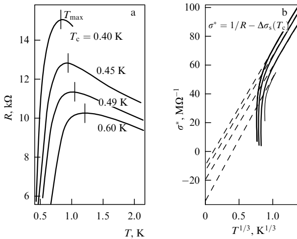
Figure 31. (a) Temperature dependences of the resistance of four TiN films in which the superconductivity is partially suppressed by disorder [114]. The meaning of the temperatures T_{\max} and T_c indicated alongside each curve is explained in the main text. For all the curves, one has T_{\max} \approx 2T_c . (b) Temperature dependences of the normal part of the conductivity, \sigma^* , for the same four films, obtained after subtracting the Aslamazov–Larkin correction with an optimum value of T_c from the total conductivity; the dashed curves have been obtained by the extrapolation of the \sigma^*(T) dependences for T \gtrsim 1 K [114].
