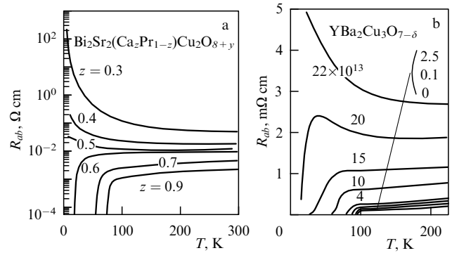
Figure 33. (a) Temperature dependences of the resistance of \text{Bi}_2\text{Sr}_2(\text{Ca}_2\text{Pr}_{1-z})\text{Cu}_2\text{O}_{8+y} samples at various Ca concentrations (indicated alongside the curves) [118]. (b) Temperature dependences of the resistance of a YBCO film after a stepped change in the dose of irradiation with \text{Ne}^+ ions [122]. The doses are indicated near the curves as the number of ions per \text{cm}^2 .
