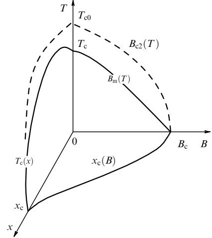
Figure 15. Region of superconducting states in the (x, B, T) space for a two-dimensional superconductor (the boundaries of the region are shown by solid curves). In an ideal system without a magnetic field ( x = B = 0 ), a superconducting transition into a resistive state occurs at a temperature T_{c0} ; at the temperature T_c , a BKT transition occurs.
