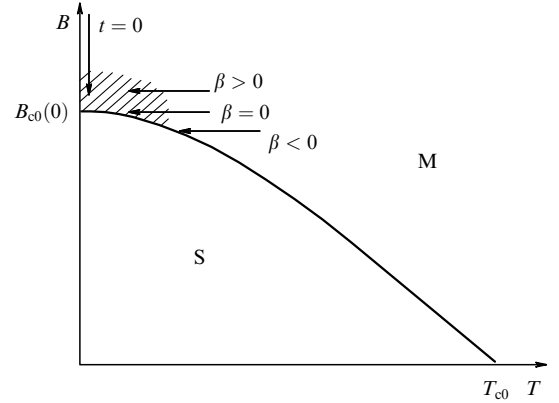
Figure 11. Phase plane (T, B) for a superconductor–dirty normal metal transition. The region of increasing resistance due to superconductor fluctuations is hatched (according to the results of calculations [59]). Arrows show different trajectories in the phase plane corresponding to different curves in Fig. 10.
