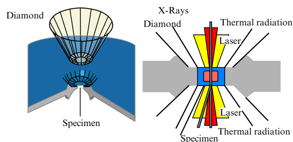
Figure 4. Schematic of a static experiment on the compression of a substance in diamond anvils involving laser heating [82].
