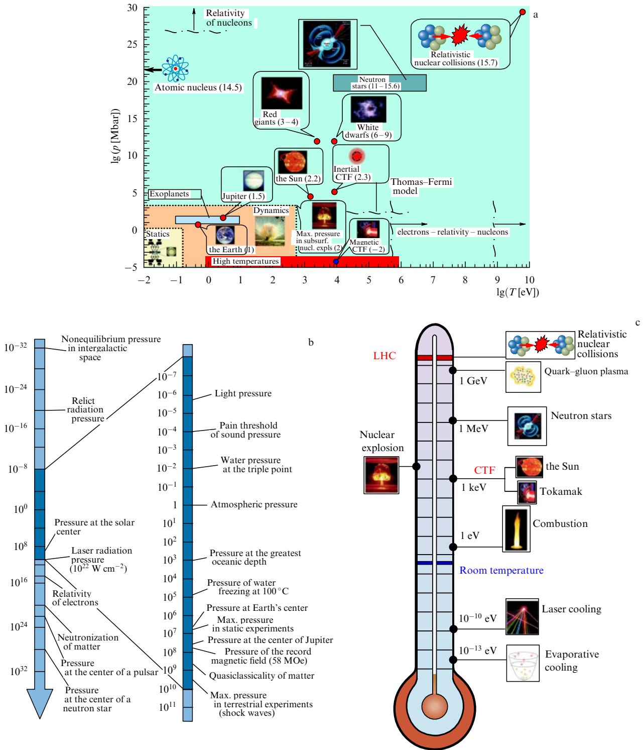
Figure 1. (a) Extreme states [1] in nature and in the laboratory. The figures in parentheses indicate the logarithm of density (in \text{g cm}^{-3} ). The domains called 'Statics' and 'Dynamics' corresponds to static and dynamic techniques for high-pressure production, and 'High temperatures' to high-temperature experiments. (b) The pressure scale range (1 atm \approx 10^5 Pa) in nature encompasses 64 orders of magnitude. The right-hand side of the scale relates to experimentally attainable conditions [18]. (c) Temperature scale.
